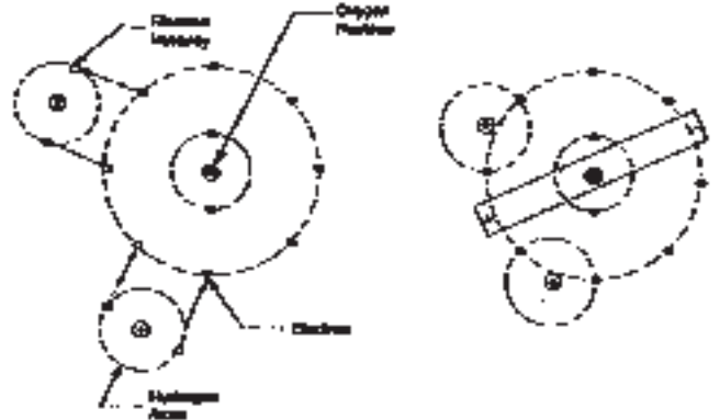
Fig. 1 — Water molecule shown as a polar molecule or a molecule with a dipole moment.
